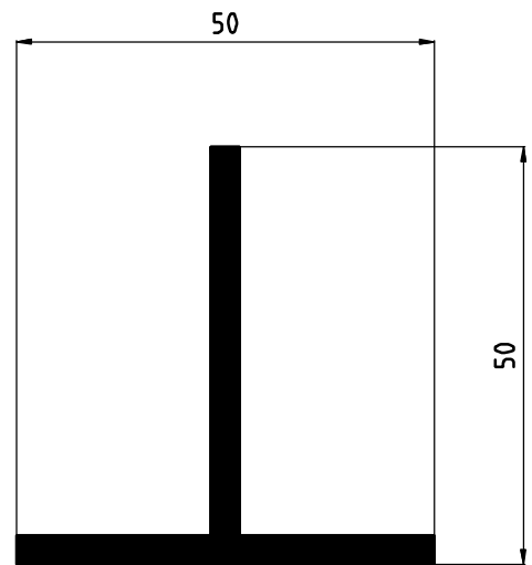
PROFILO T BST0917 1,282 Kg/ml
