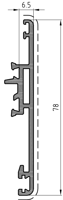
BBC1482 24860 0.730Kg/m GUSCIO
